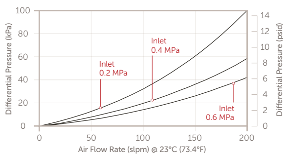
Gasketgard – ⅜" Fittings
