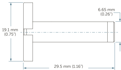
½" (⅜") Gasket Seal with Retainer
