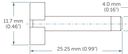
¼" Gasket Seal with Retainer
