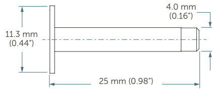
¼" Gasket Seal
