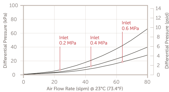
Gasketgard – ¼" Fittings
