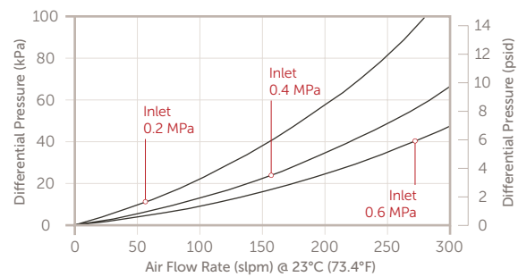
Gasketgard – ½" Fittings
